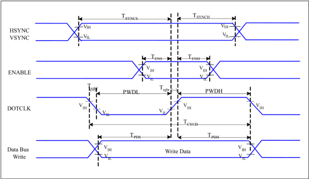
RGB Interface Timing Characteristics
