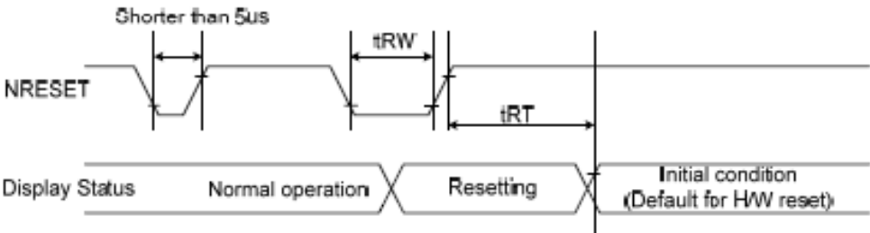
Figure 102 Reset Timing
