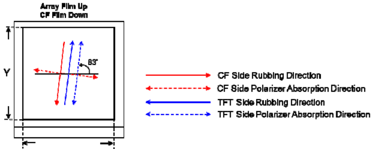
Note (5) Rubbing Direction & Polarizer Absorption Direction
