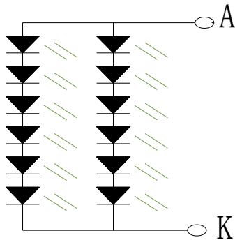
Backlight LED Circuit
