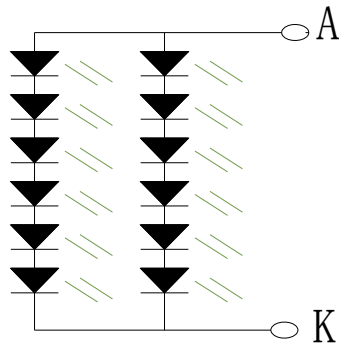
Backlight LED Circuit
