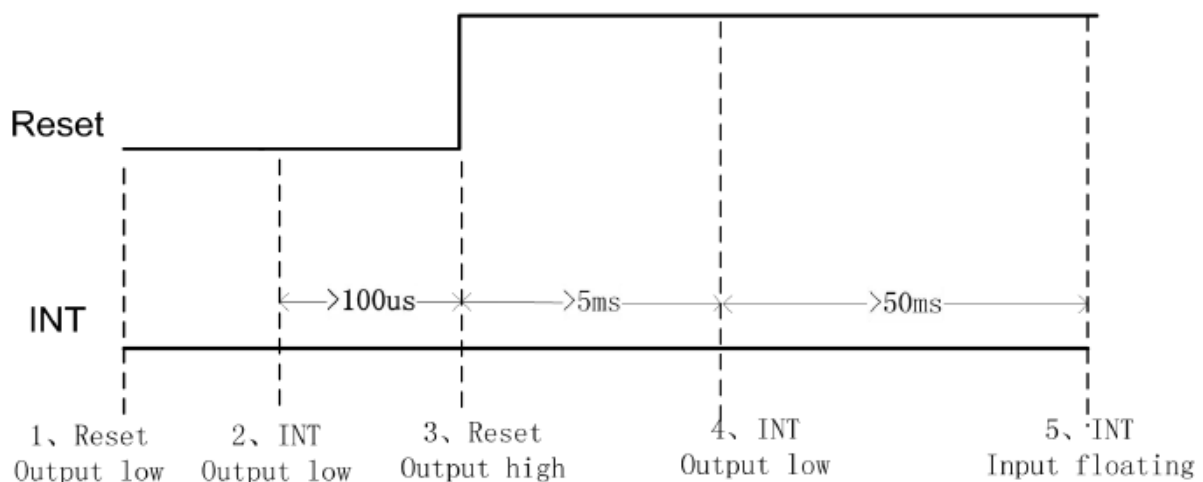
Timing for setting slave address to 0xBA/0xBB:
